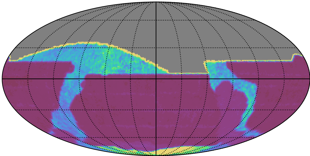
baseline_v3.5_10yrs All sky all bands: Median Inter-Night Gap
