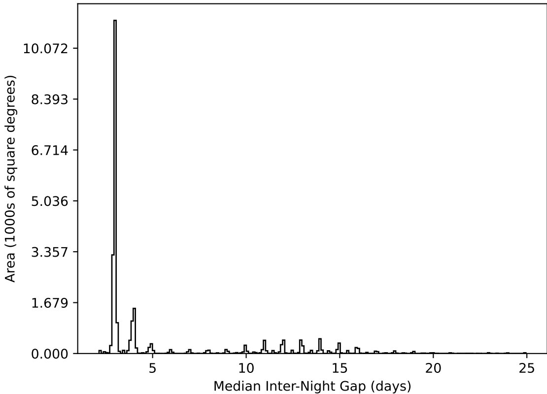
baseline_v3.5_10yrs All sky all bands: Median Inter-Night Gap
