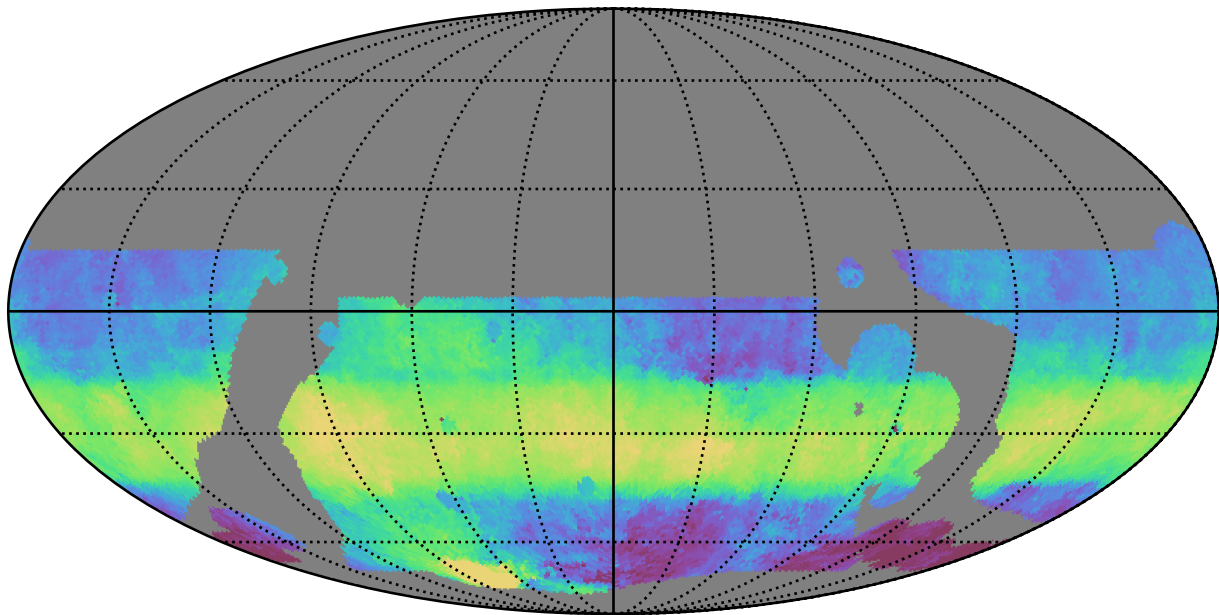
baseline_v3.5_10yrs WFD z band: Median HA
