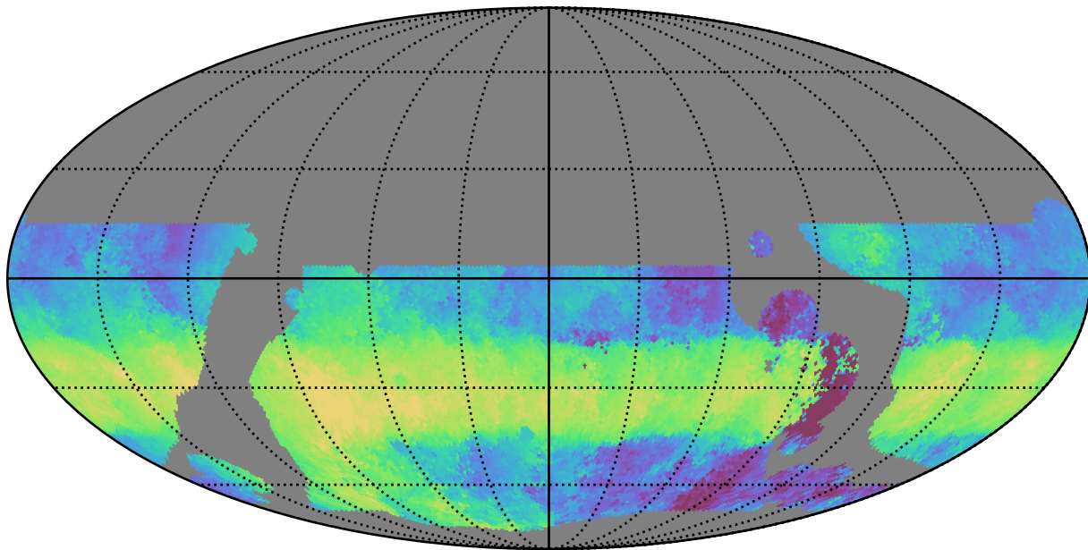
baseline_v3.5_10yrs WFD u band: Median HA
