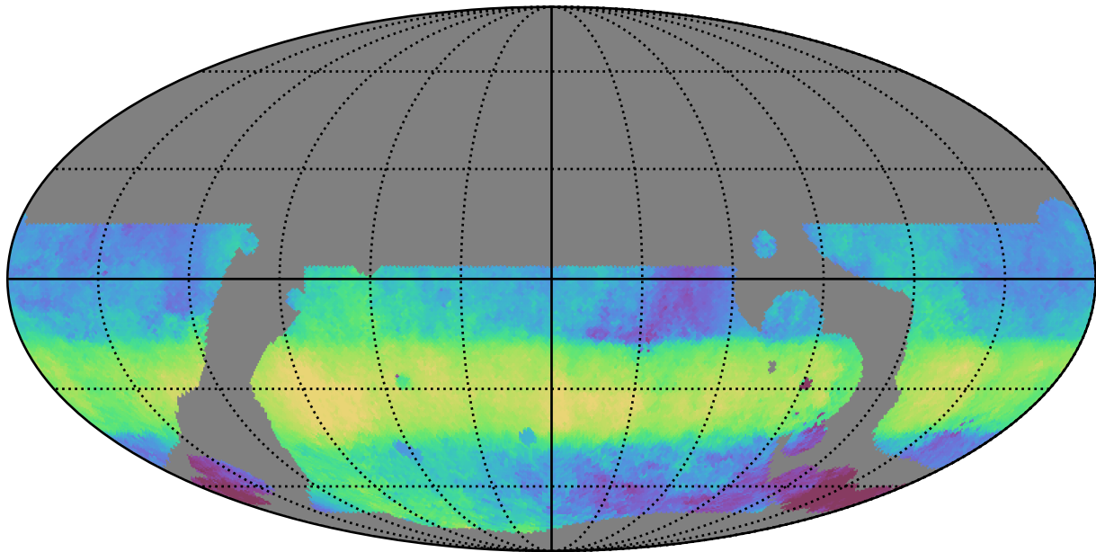
baseline_v3.5_10yrs WFD r band: Median HA
