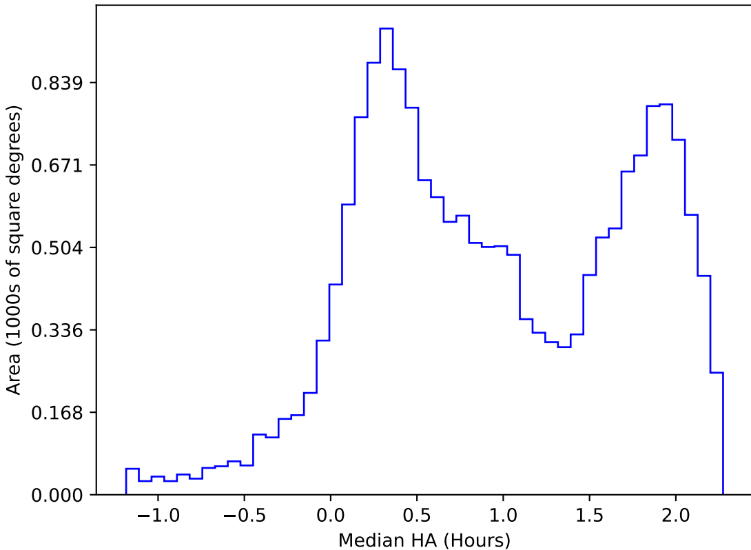
baseline_v3.5_10yrs WFD i band: Median HA
