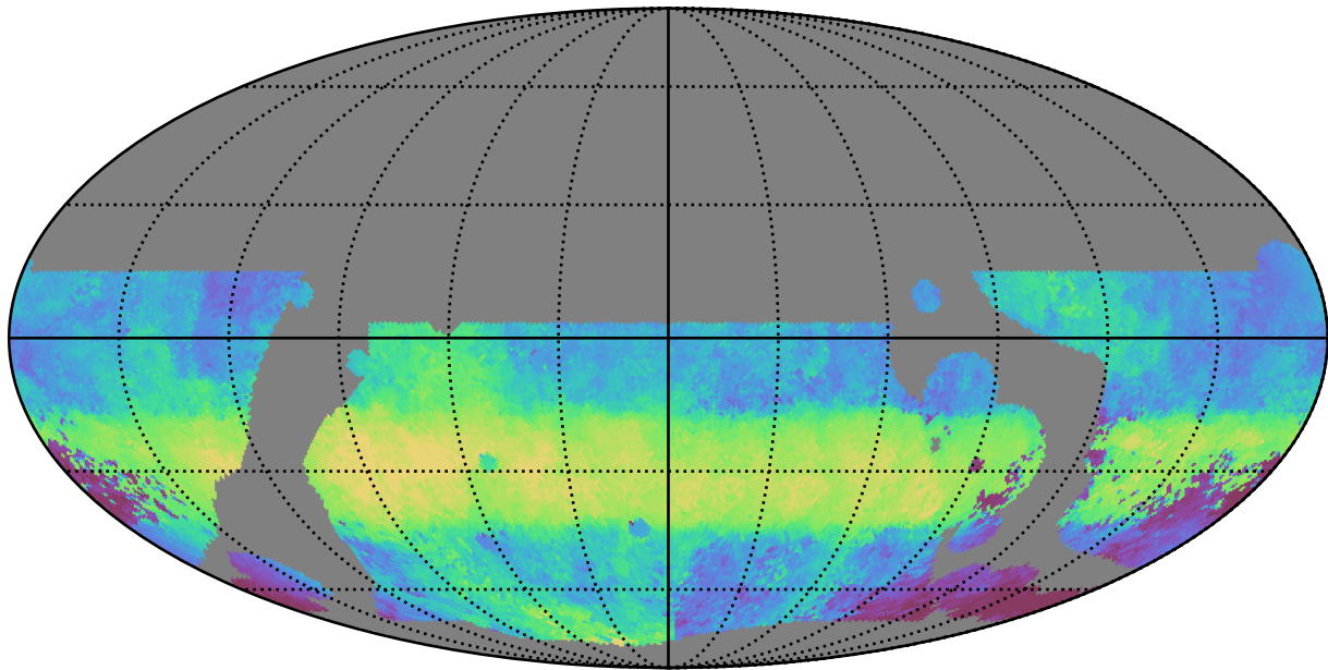
baseline_v3.5_10yrs WFD g band: Median HA
