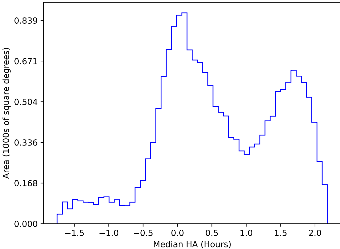
baseline_v3.5_10yrs WFD g band: Median HA
