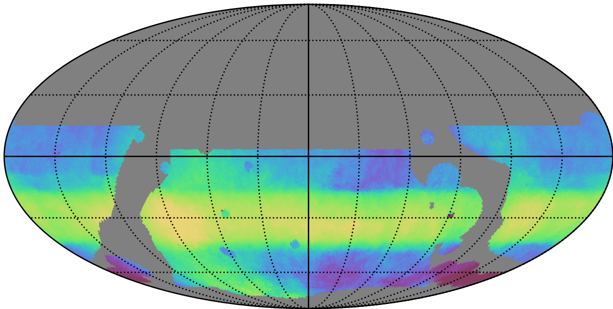
baseline_v3.5_10yrs WFD all bands: Median HA
