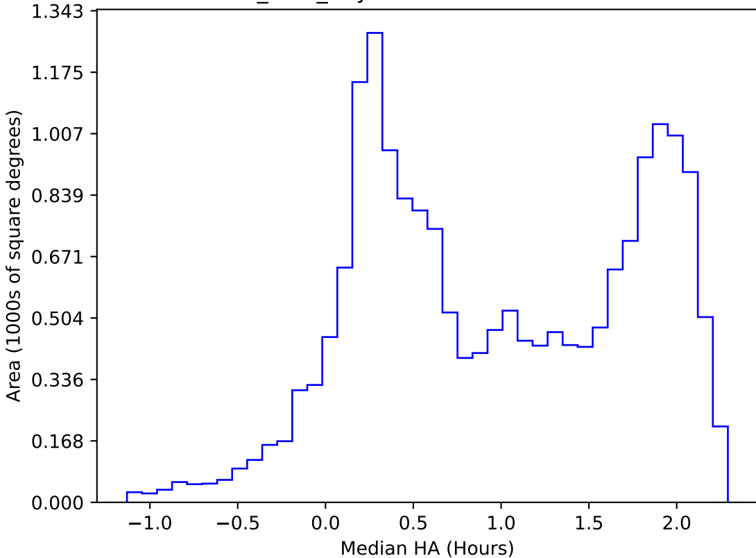
baseline_v3.5_10yrs WFD all bands: Median HA
