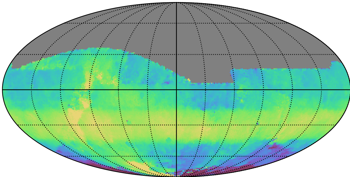
baseline_v3.5_10yrs All sky z band: Median HA
