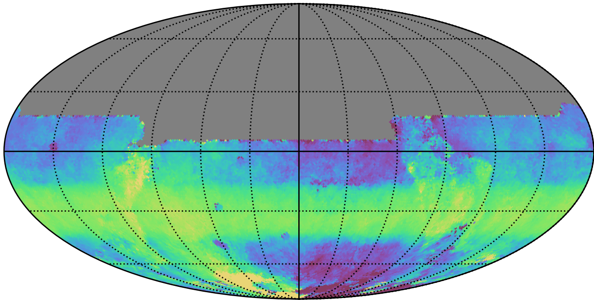
baseline_v3.5_10yrs All sky y band: Median HA
