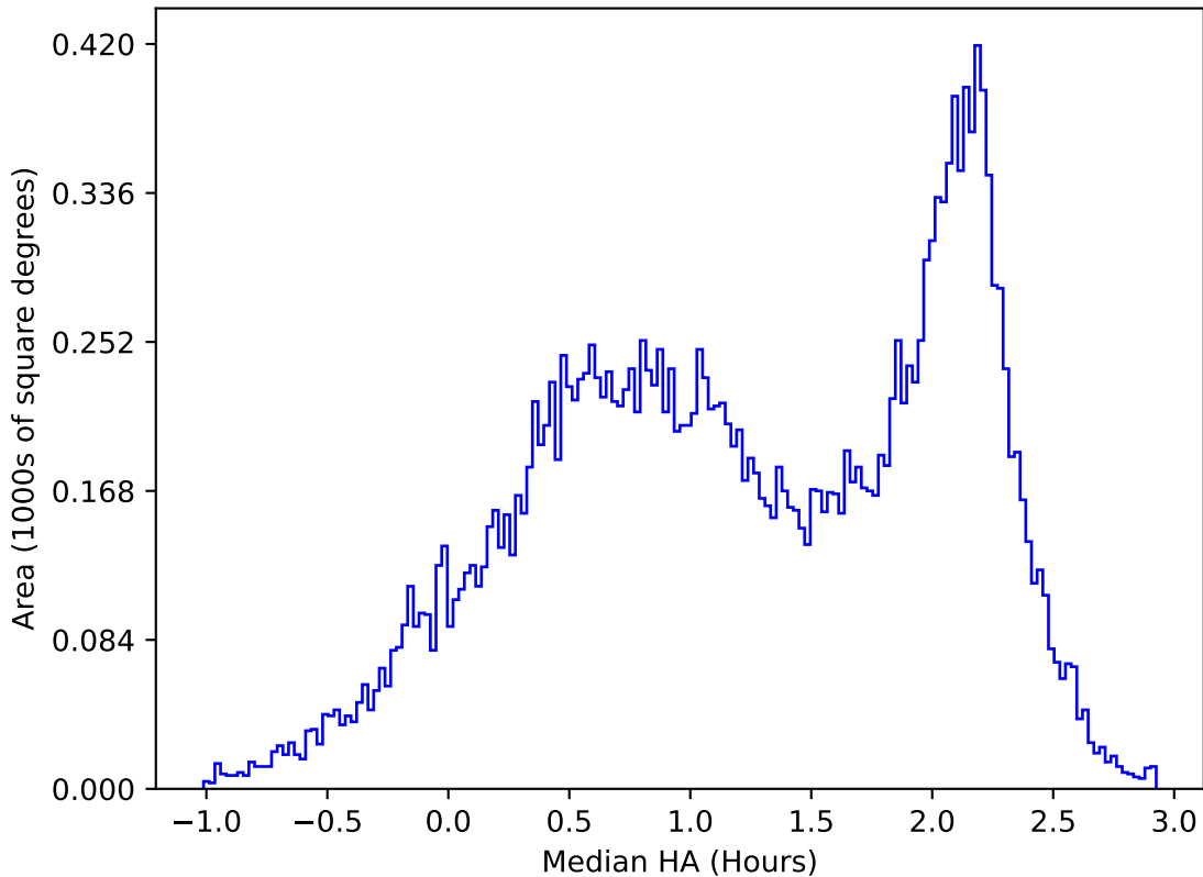
baseline_v3.5_10yrs All sky y band: Median HA
