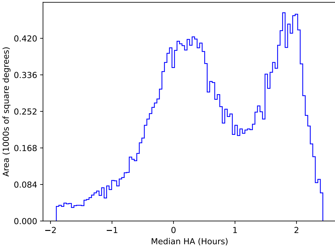
baseline_v3.5_10yrs All sky u band: Median HA
