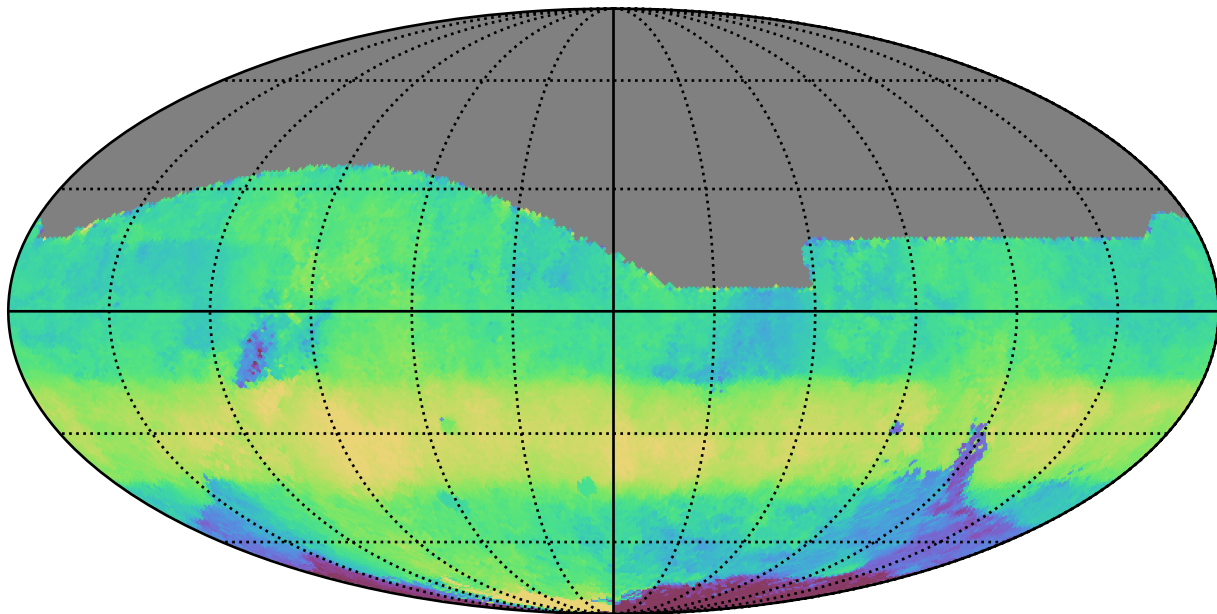
baseline_v3.5_10yrs All sky r band: Median HA
