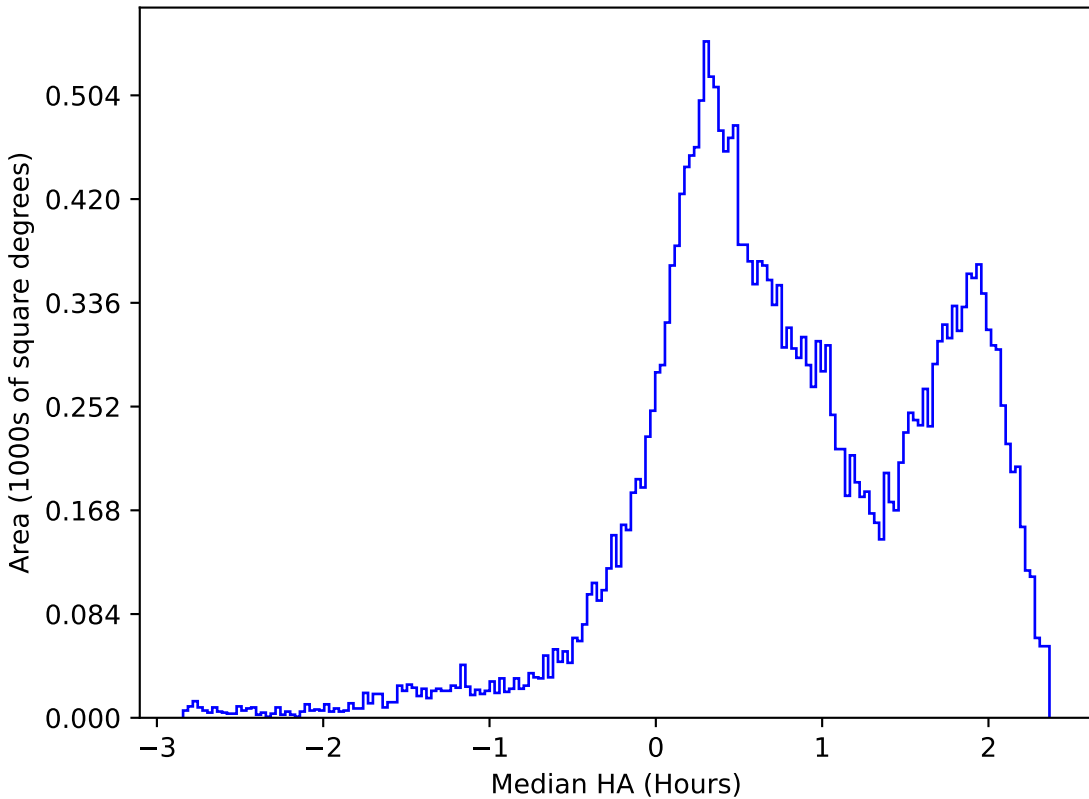
baseline_v3.5_10yrs All sky i band: Median HA
