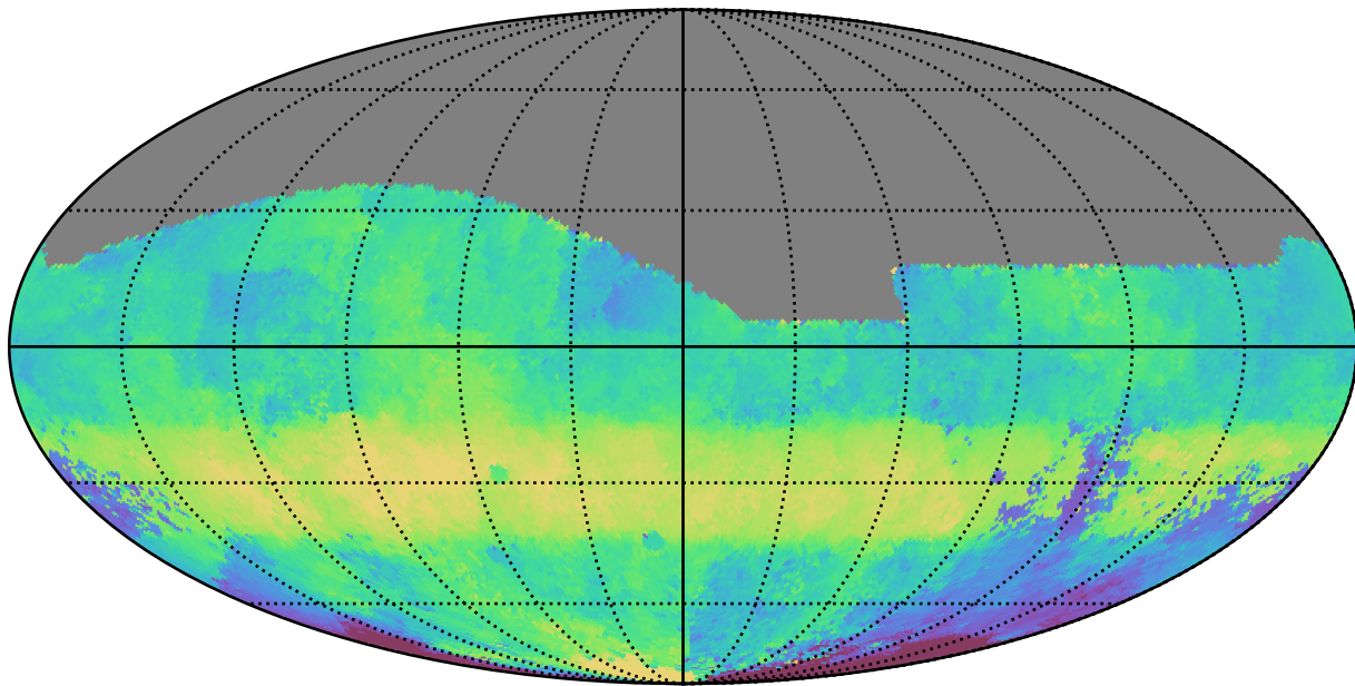
baseline_v3.5_10yrs All sky g band: Median HA
