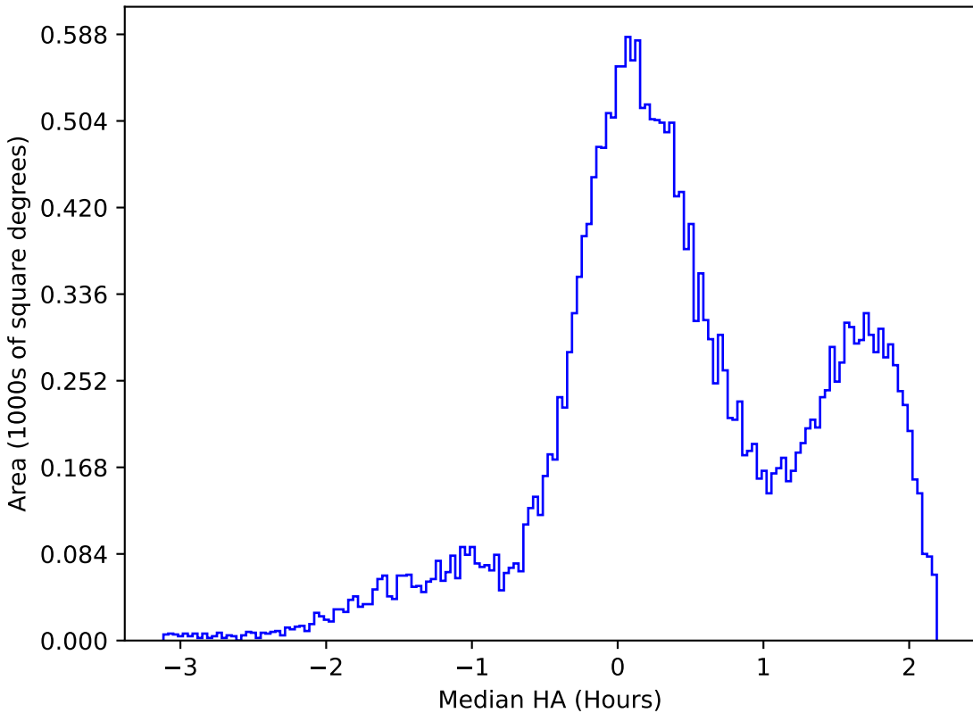
baseline_v3.5_10yrs All sky g band: Median HA
