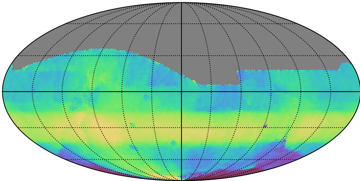
baseline_v3.5_10yrs All sky all bands: Median HA
