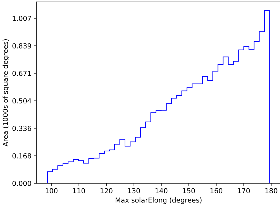
baseline_v3.5_10yrs WFD z band: Max solarElong
