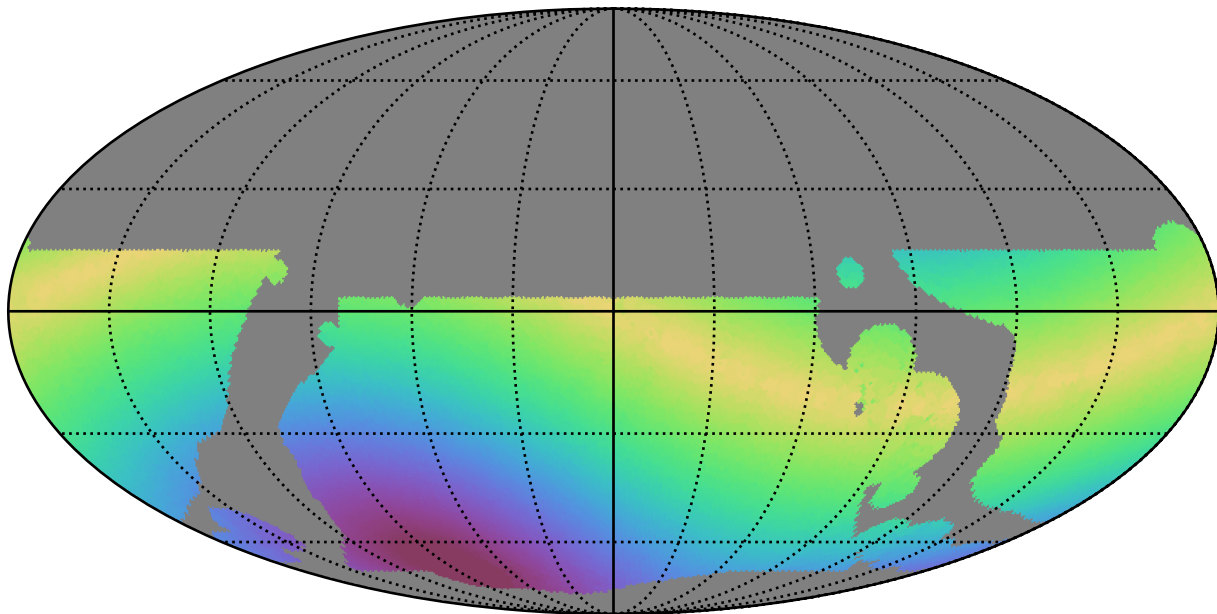
baseline_v3.5_10yrs WFD y band: Max solarElong
