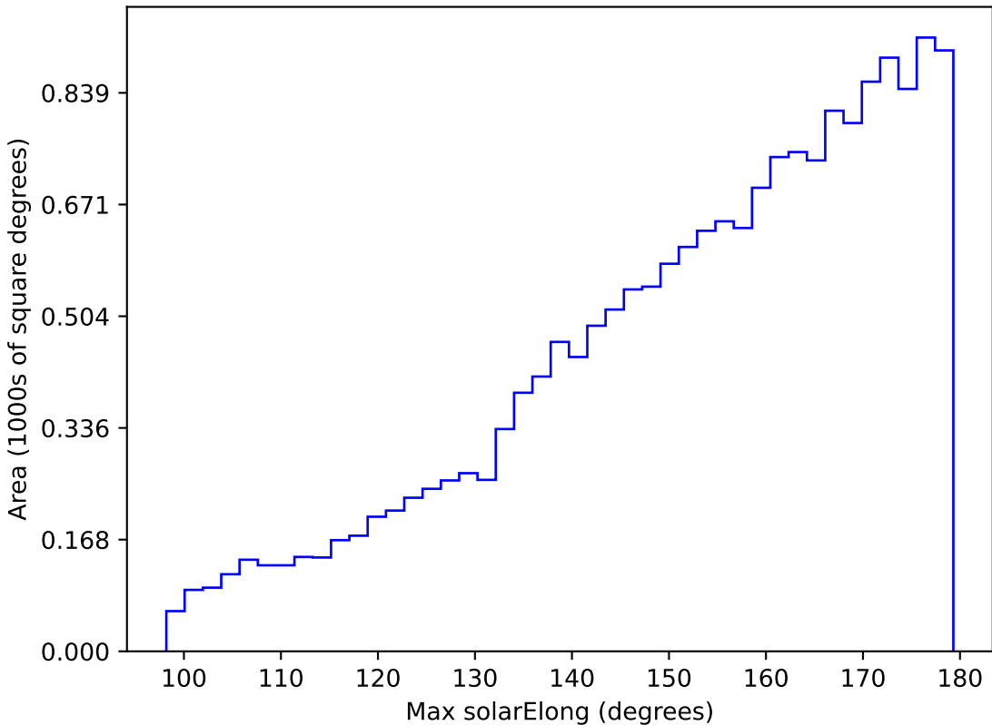
baseline_v3.5_10yrs WFD y band: Max solarElong
