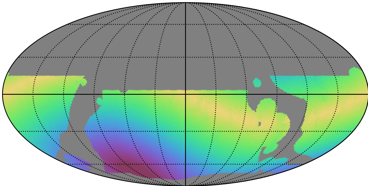
baseline_v3.5_10yrs WFD u band: Max solarElong
