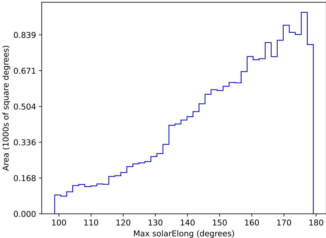
baseline_v3.5_10yrs WFD u band: Max solarElong
