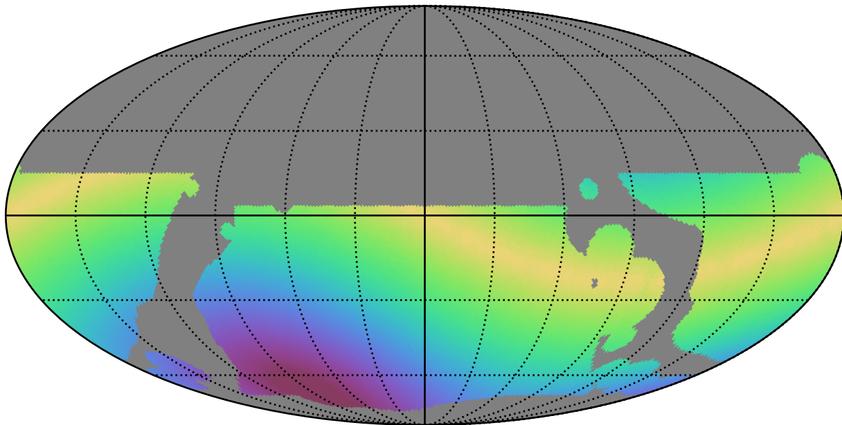
baseline_v3.5_10yrs WFD r band: Max solarElong
