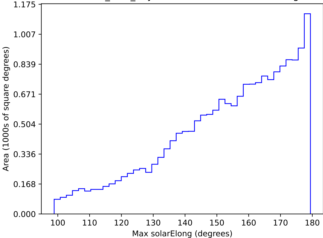
baseline_v3.5_10yrs WFD r band: Max solarElong
