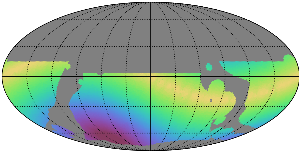
baseline_v3.5_10yrs WFD g band: Max solarElong
