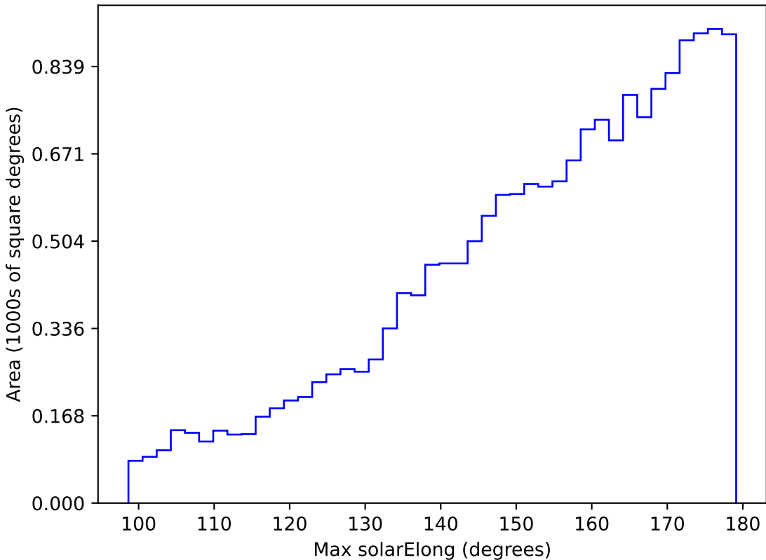
baseline_v3.5_10yrs WFD g band: Max solarElong
