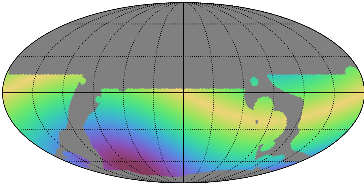
baseline_v3.5_10yrs WFD all bands: Max solarElong
