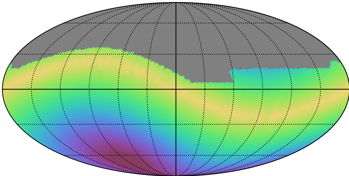
baseline_v3.5_10yrs All sky z band: Max solarElong
