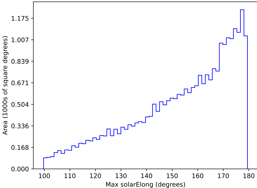
baseline_v3.5_10yrs All sky z band: Max solarElong
