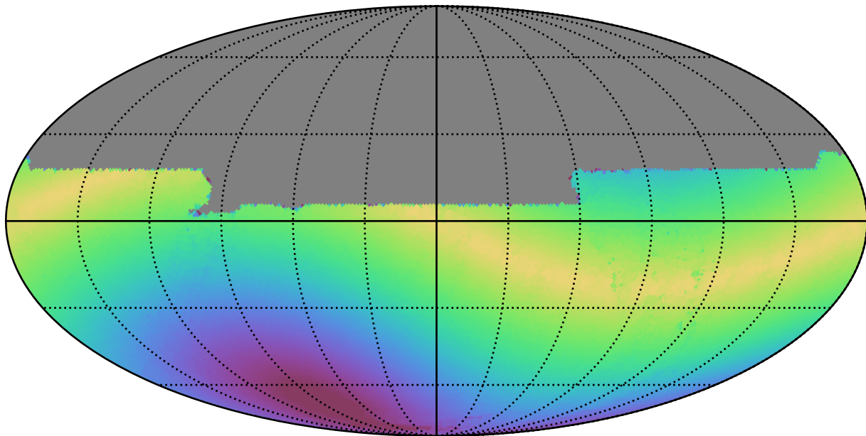
baseline_v3.5_10yrs All sky y band: Max solarElong
