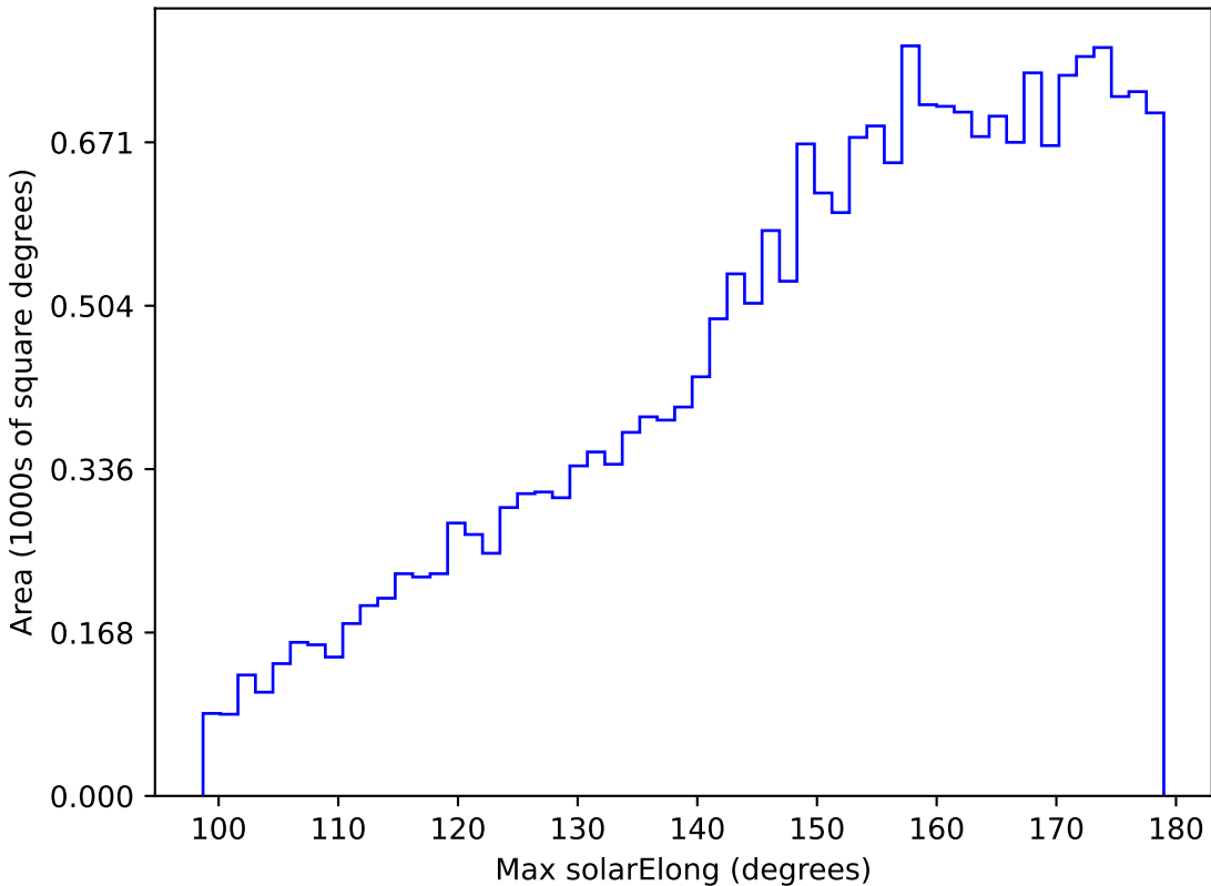
baseline_v3.5_10yrs All sky u band: Max solarElong
