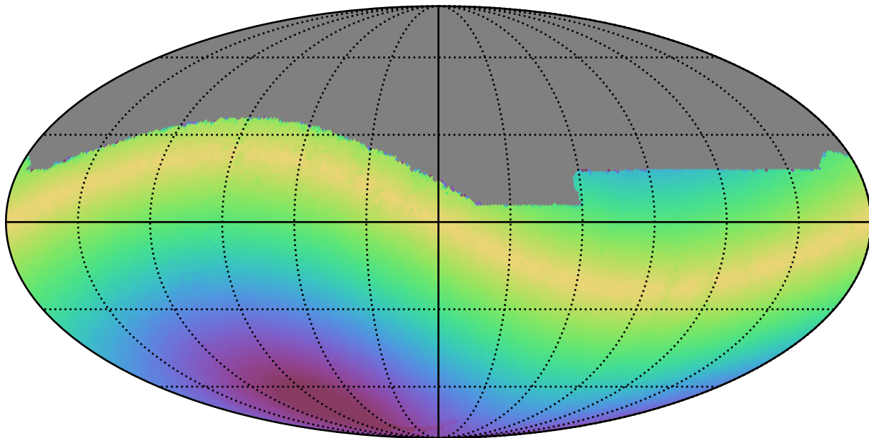
baseline_v3.5_10yrs All sky r band: Max solarElong
