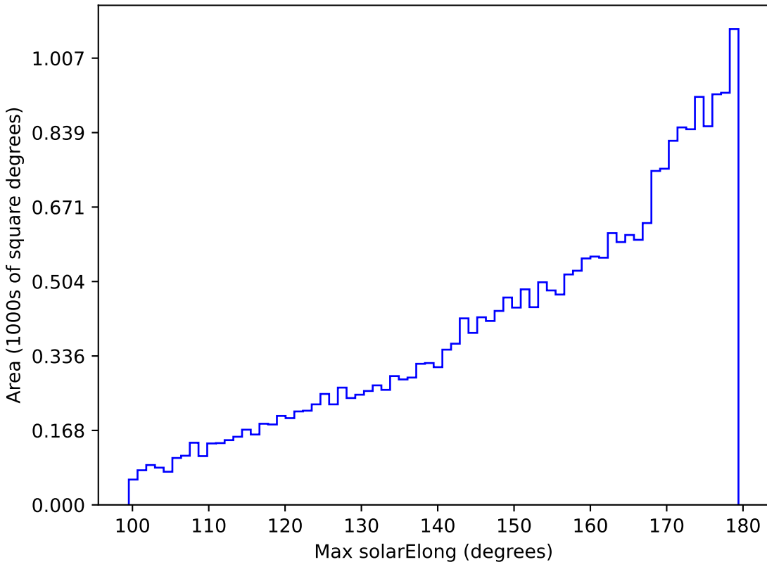
baseline_v3.5_10yrs All sky r band: Max solarElong
