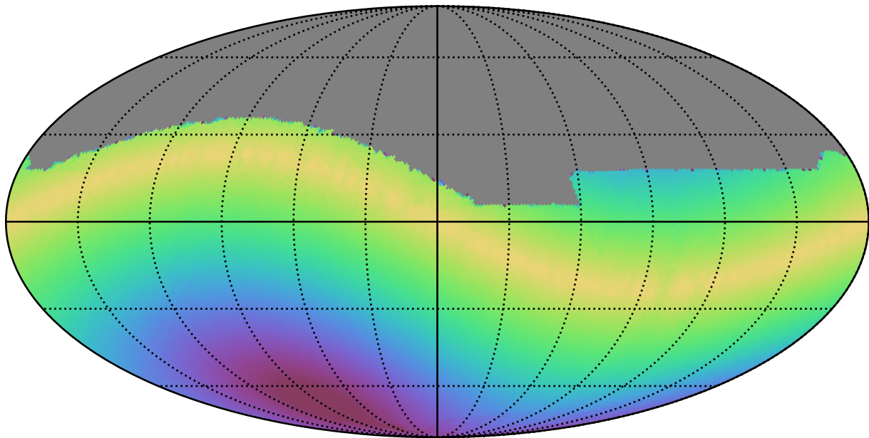
baseline_v3.5_10yrs All sky i band: Max solarElong
