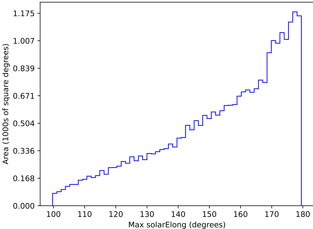
baseline_v3.5_10yrs All sky i band: Max solarElong
