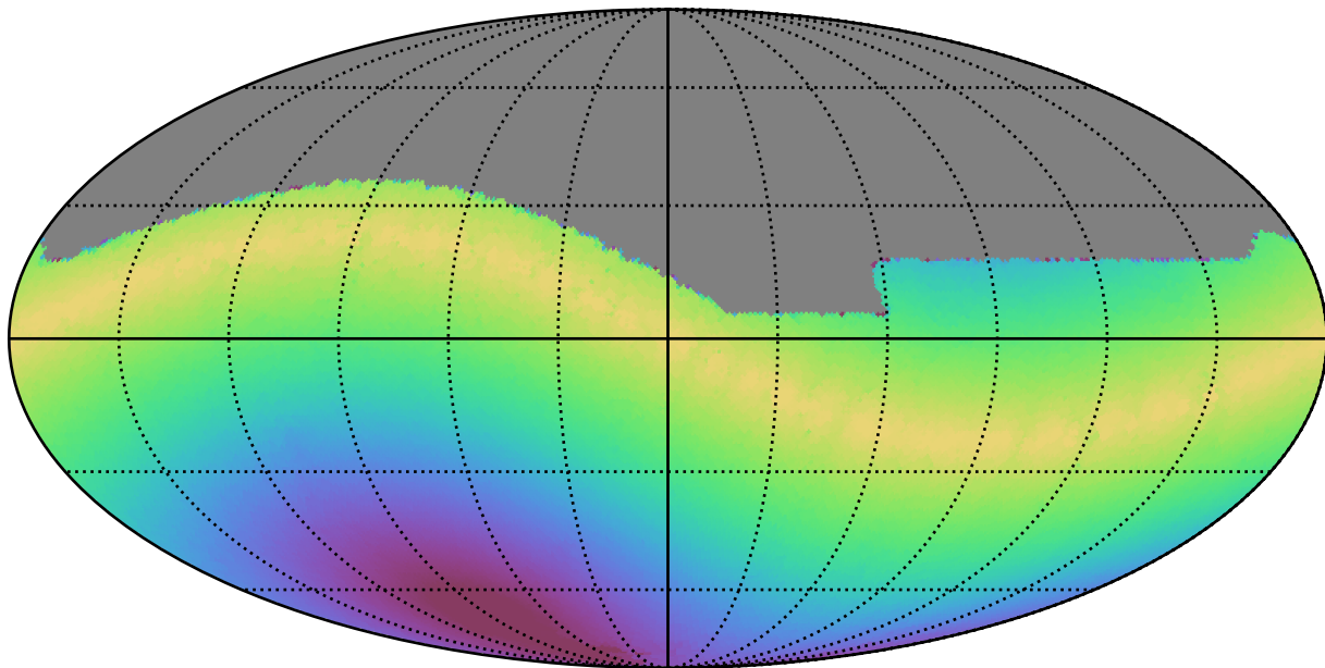
baseline_v3.5_10yrs All sky g band: Max solarElong
