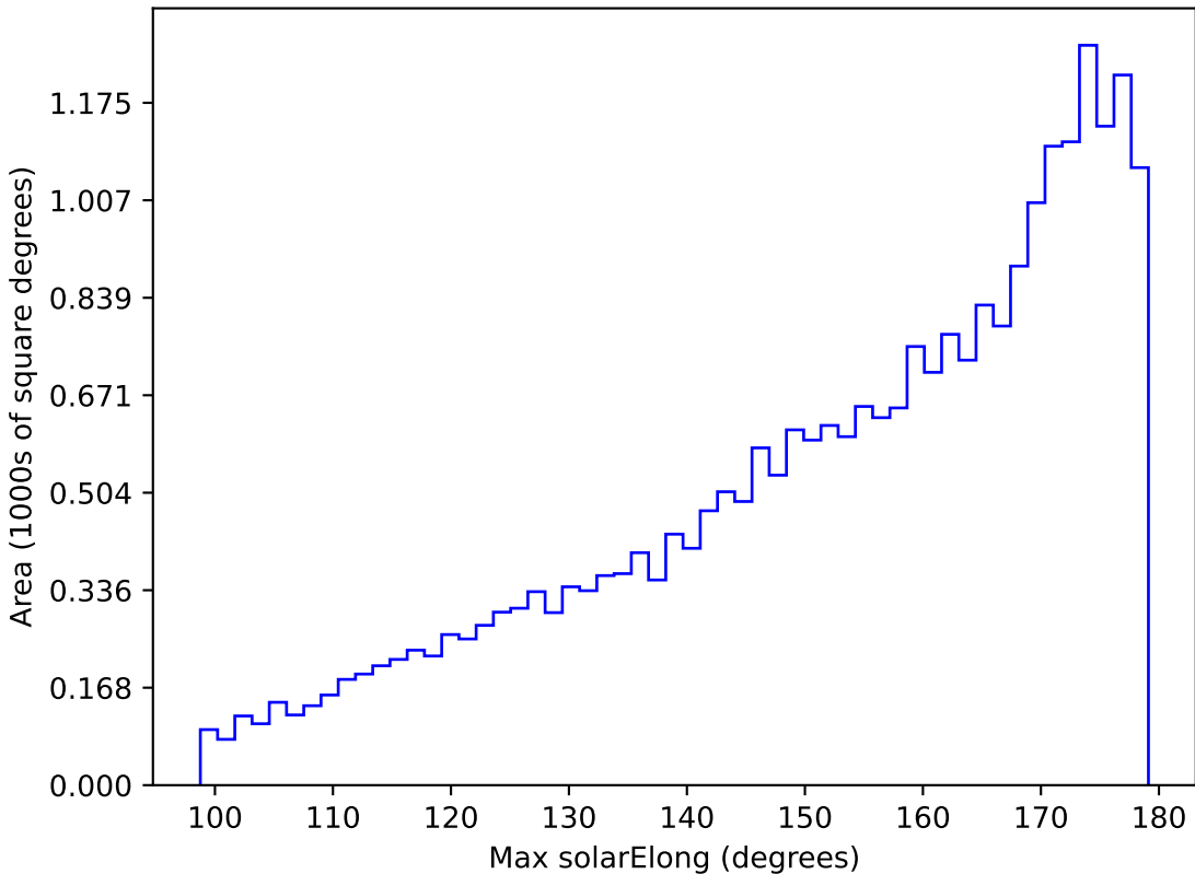
baseline_v3.5_10yrs All sky g band: Max solarElong
