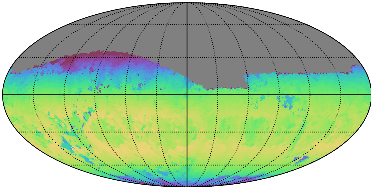
baseline_v3.5_10yrs Yr 1 z band: Max skyBrightness
