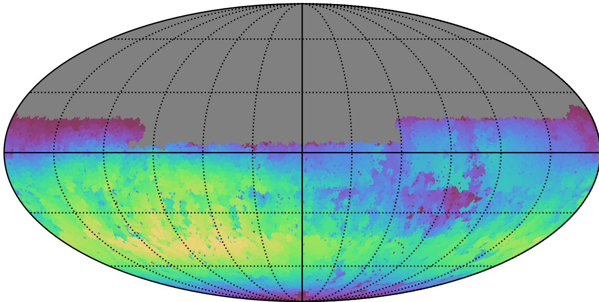
baseline_v3.5_10yrs Yr 1 u band: Max skyBrightness
