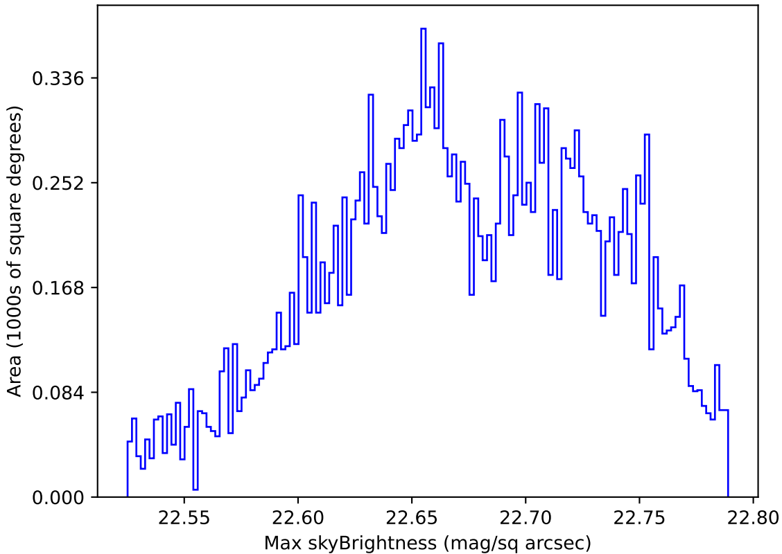
baseline_v3.5_10yrs Yr 1 u band: Max skyBrightness
