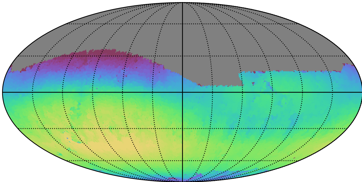
baseline_v3.5_10yrs Yr 1 r band: Max skyBrightness
