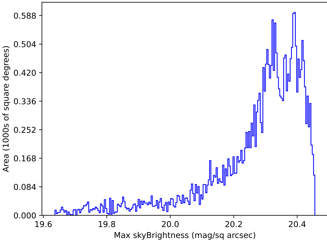
baseline_v3.5_10yrs Yr 1 i band: Max skyBrightness
