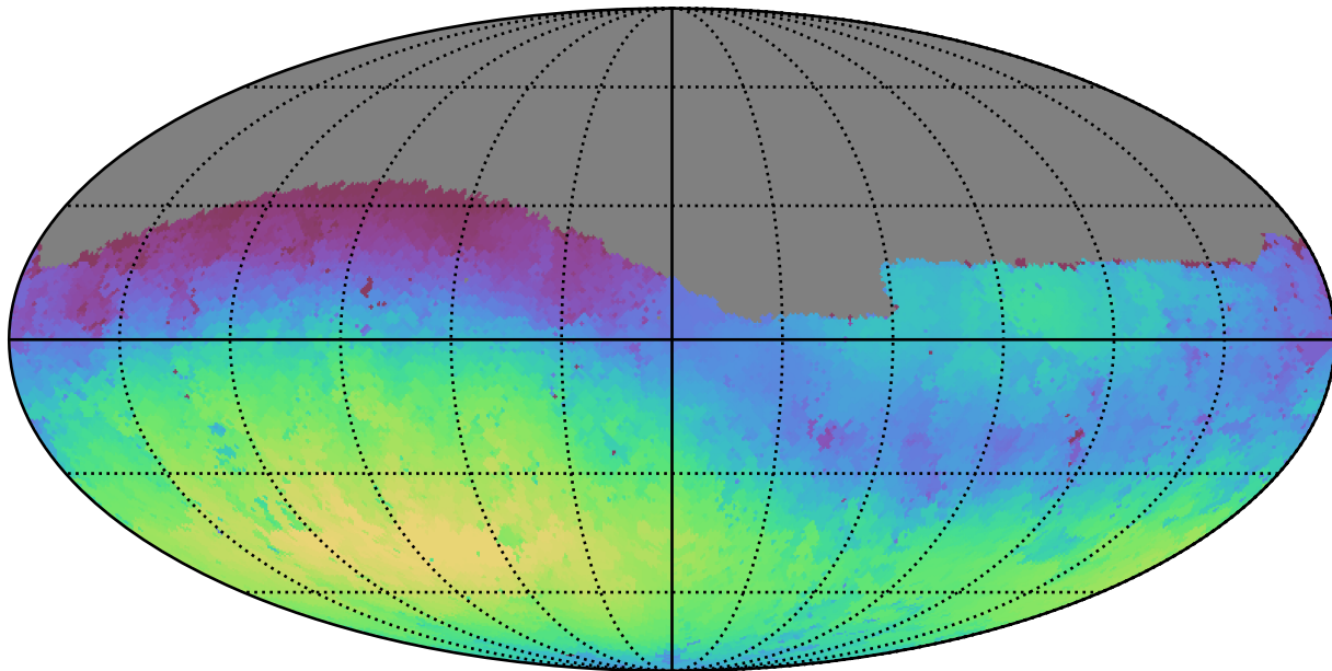
baseline_v3.5_10yrs Yr 1 g band: Max skyBrightness
