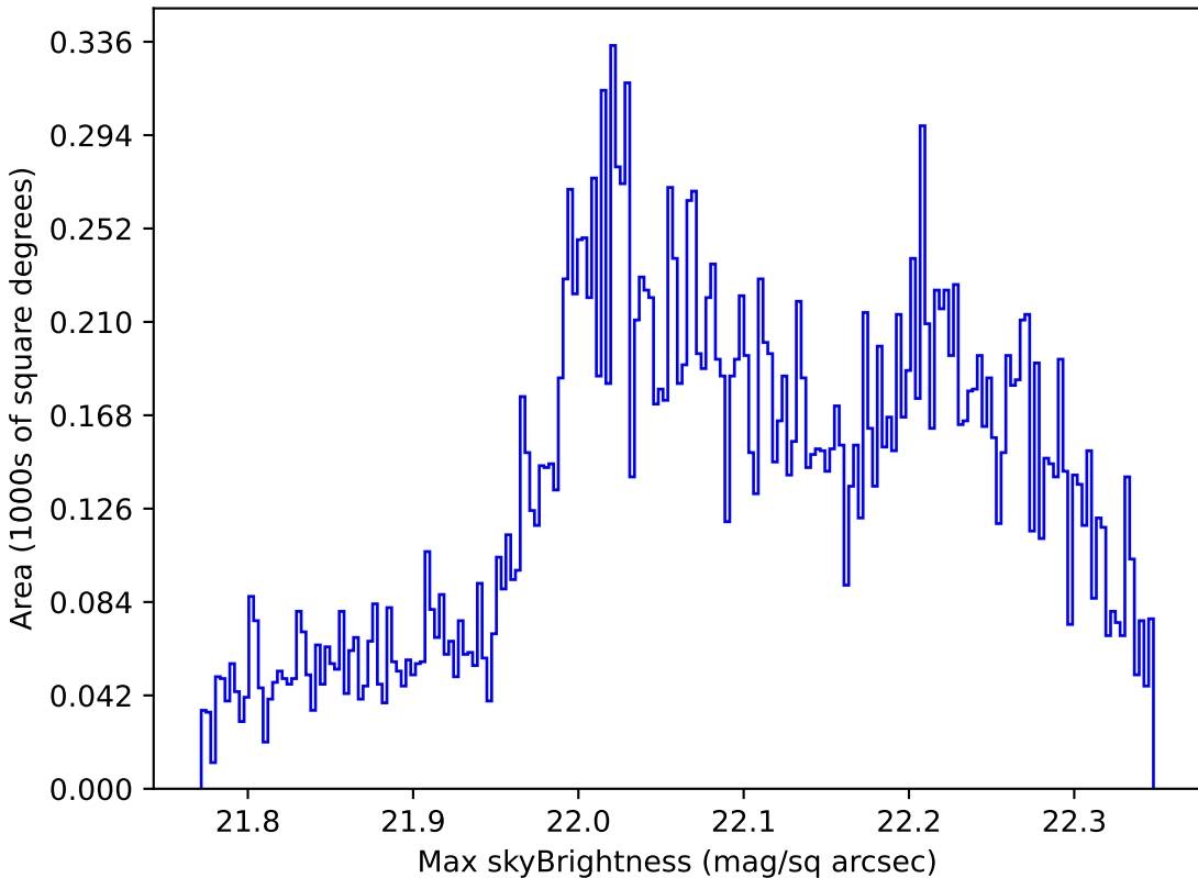
baseline_v3.5_10yrs Yr 1 g band: Max skyBrightness
