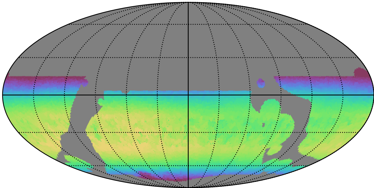
baseline_v3.5_10yrs WFD z band: Max skyBrightness
