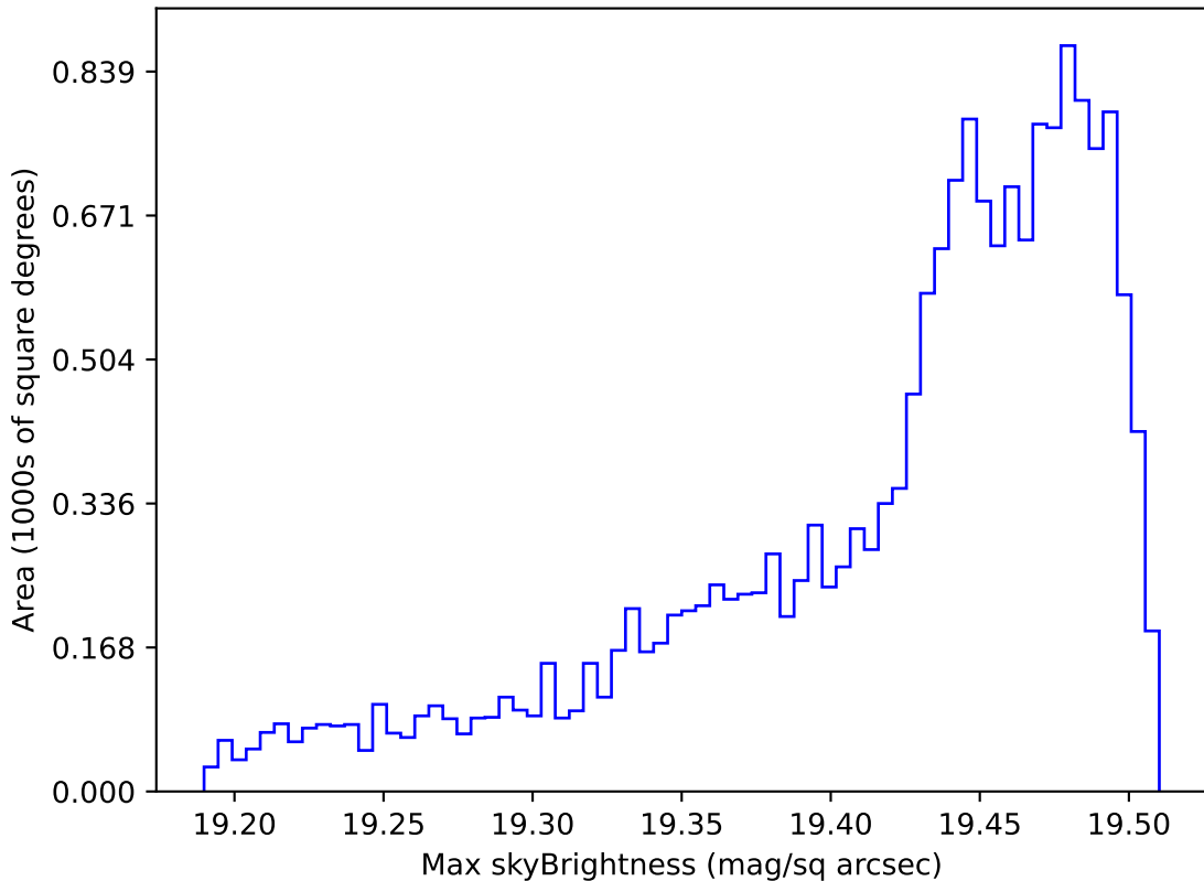
baseline_v3.5_10yrs WFD z band: Max skyBrightness
