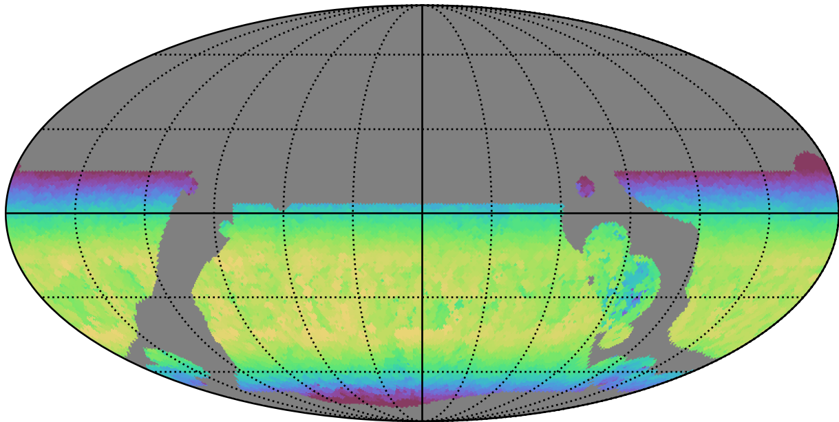
baseline_v3.5_10yrs WFD y band: Max skyBrightness
