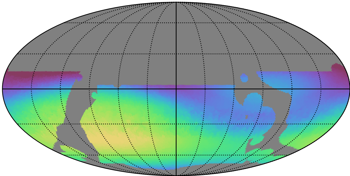
baseline_v3.5_10yrs WFD r band: Max skyBrightness
